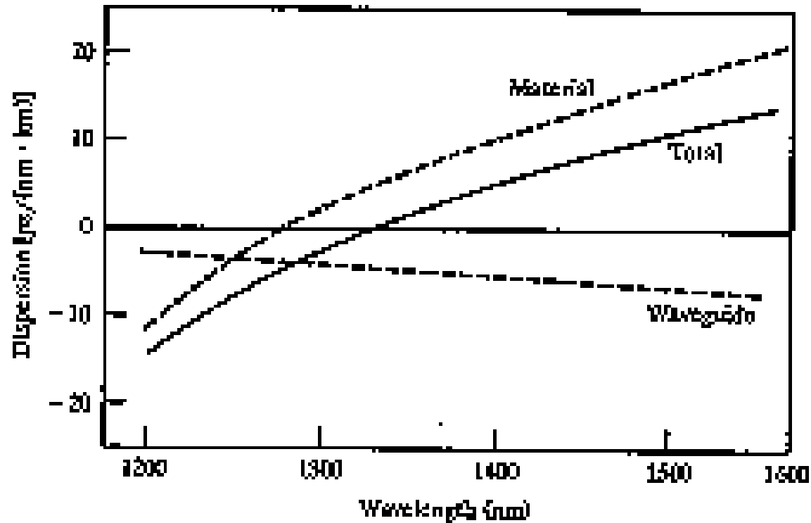
FIGURE 3-16 Examples of the magnitudes of material and waveguide dispersion as a function of optical wavelength for a single-mode fused-silica-core fiber. (Reproduced with permission from Keck, 16 © 1985, IEEE.)
